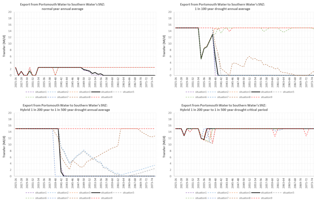
Figure 16: Utilisation of bulk import from Portsmouth Water to Southern Water’s SNZ with the volume capped at 2.5Ml/d under normal year conditions.
