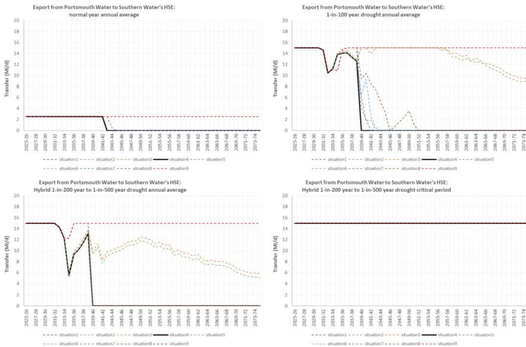
Figure 15: Utilisation of the export from Portsmouth Water to Southern Water’s HSE with supply under normal year conditions restricted to 2.5Ml/d.
